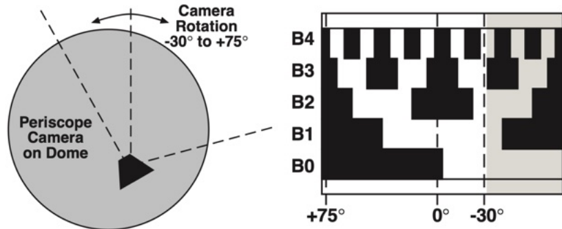
Instrumentation for Gray Scale Encoder
